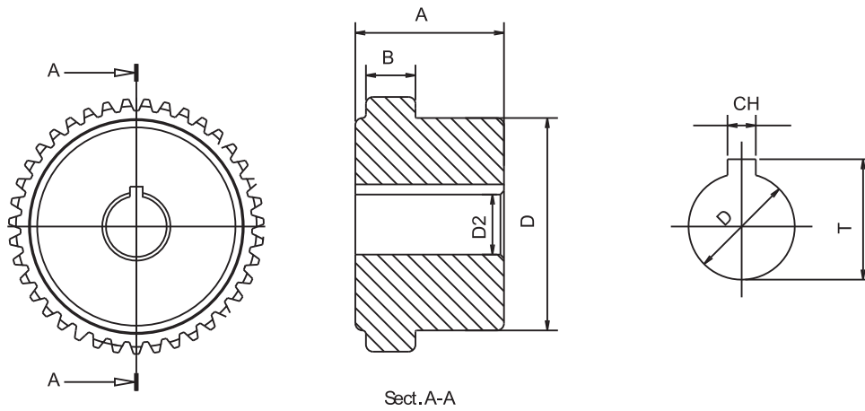
Sect. A-A
