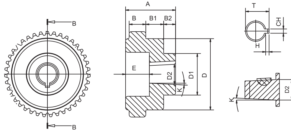
Sect. B-B
